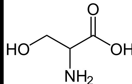
Serine
