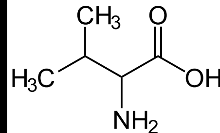
Valine
