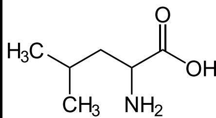
Leucine
