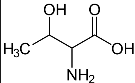
Threonine
