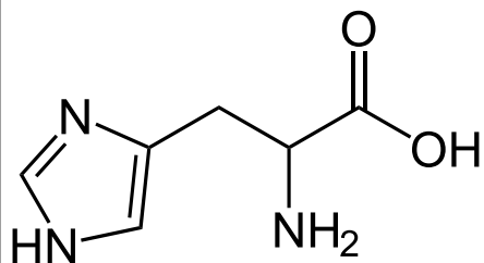
Histidine
