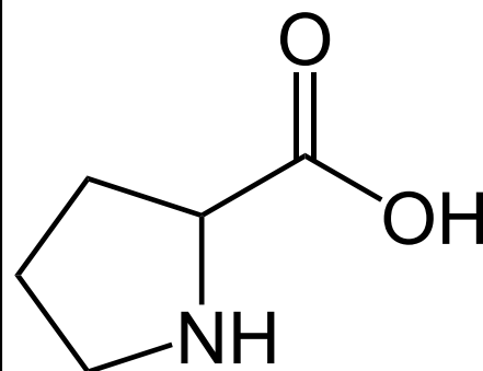
Proline
