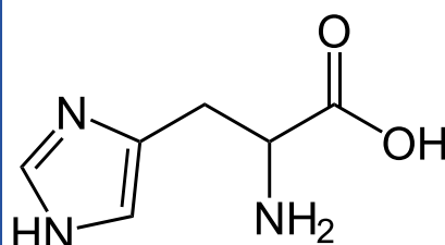
Histidine
