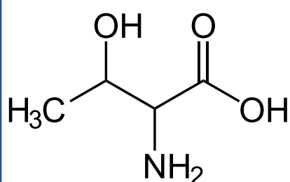
Threonine
