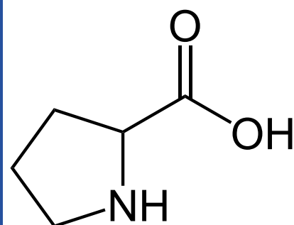
Proline
