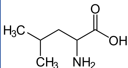
Leucine
