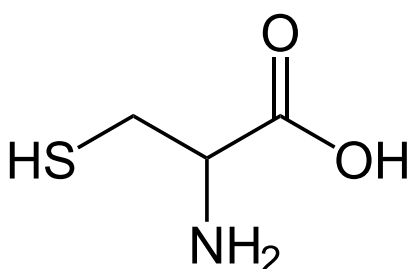
Cysteine
