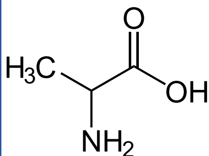
Alanine
