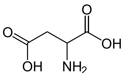
Aspartic acid
