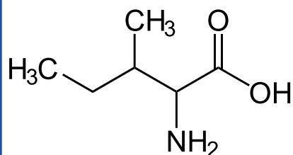
Isoleucine
