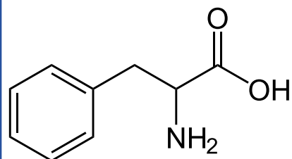
Phenylalanine
