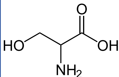
Serine
