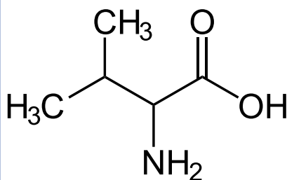
Valine
