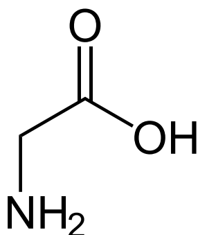
Glycine
