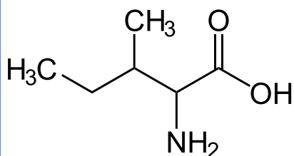
Isoleucine
