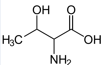
Threonine
