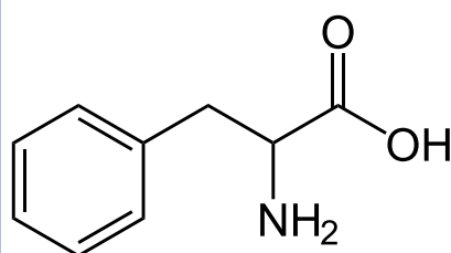
Phenylalanine
